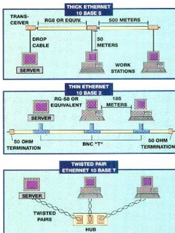
Figure 1. Equipment and wiring layouts for various network configurations.
