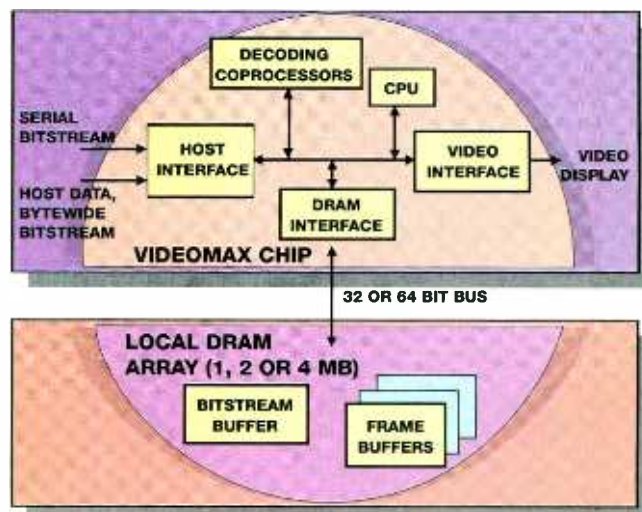
Figure 1. Simplified block diagram and external interfaces of the Videomax (CL9100) chip.
